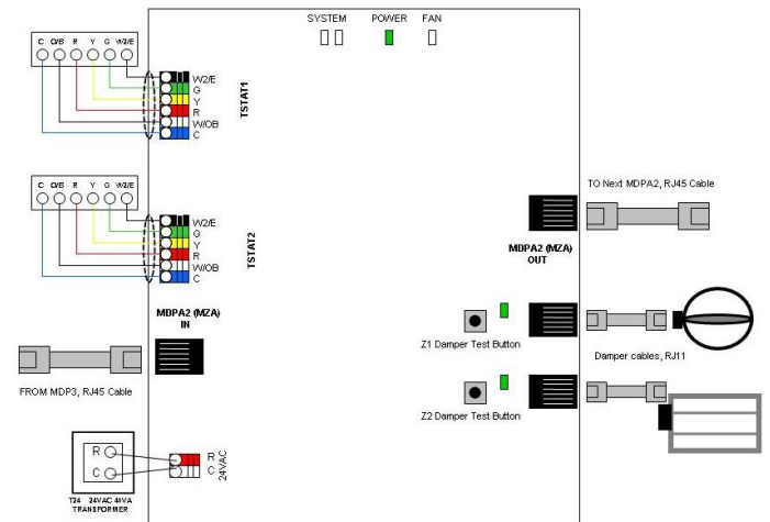
MDPA2 Panel Wiring Diagram
